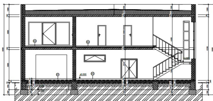
REZ A - A
